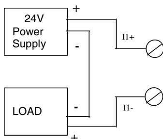
Current Source
