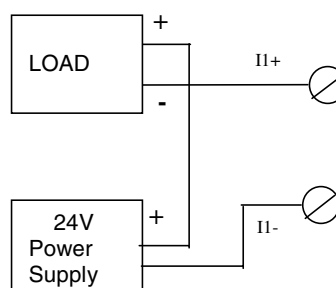
Current Sink
