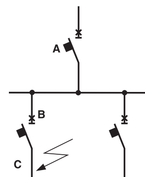
Circuit diagram with selective coordination of protections
