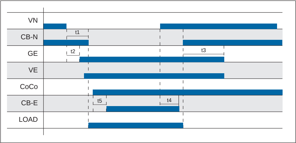
Caption VN Network voltage CB-N Normal line circuit-breaker closed GE Generator VE Emergency line voltage CoCo Enabling switching to emergency line CB-E Emergency line circuit-breaker closed LOAD Disconnection of lower priority loads
