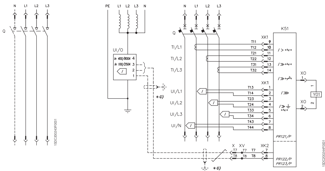
Four-pole circuit-breaker with PR121/P, PR122/P or PR123/P electronic trip unit
