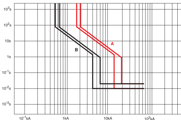
Example of current-type selectivity
