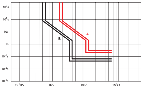
Example of time-type selectivity
