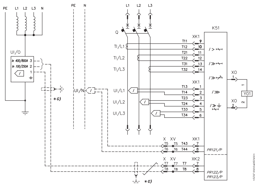
Three-pole circuit-breaker with PR121/P, PR122/P or PR123/P electronic trip unit
